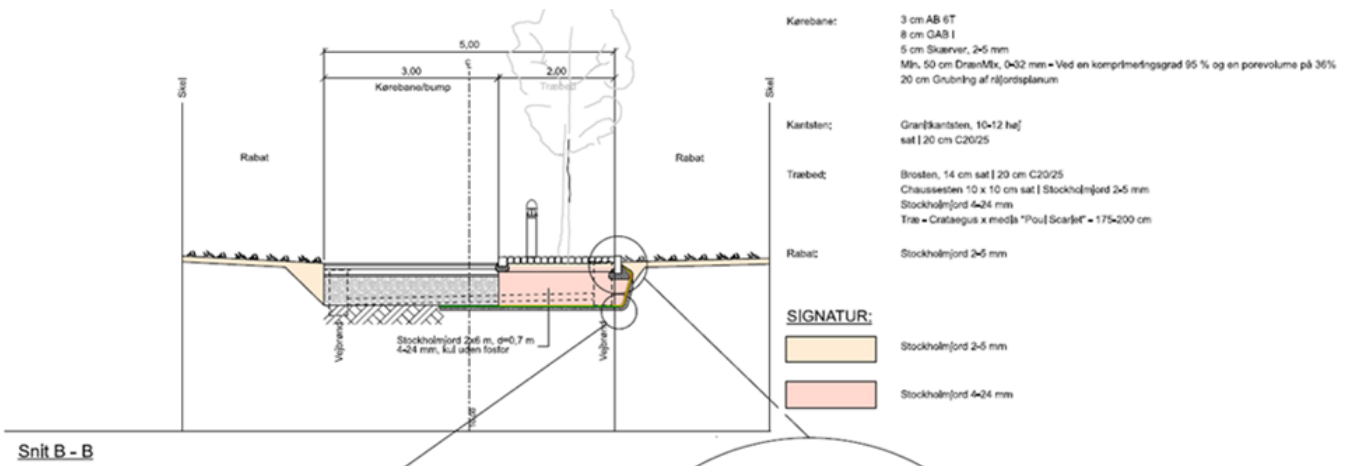
Snit B - B
