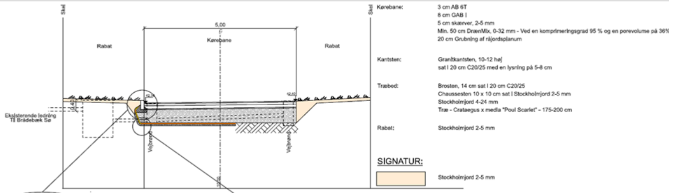
Snit A - A
